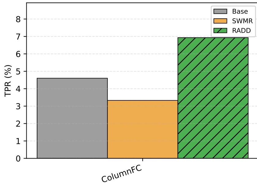
LiRA TPR@0.5%FPR
