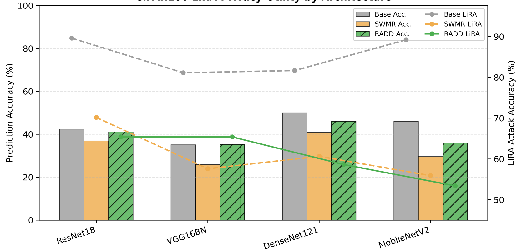
CIFAR100 LiRA Privacy-Utility by Architecture
