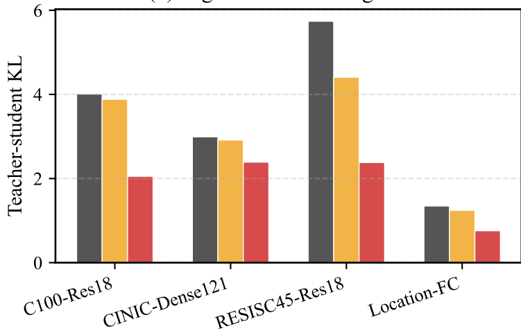
(b) High-risk teacher alignment
