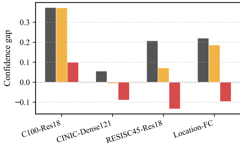
(a) High-risk confidence gap
