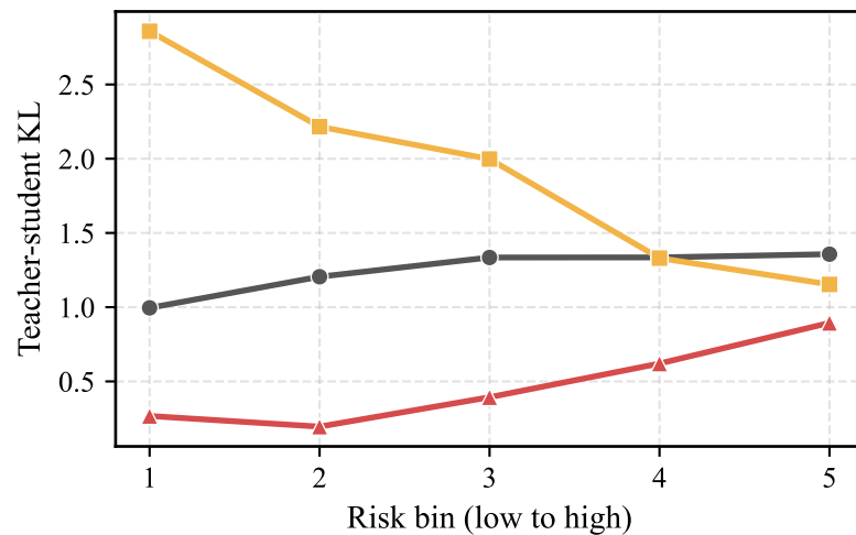
Location FC
