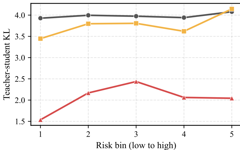
CIFAR100 ResNet18
