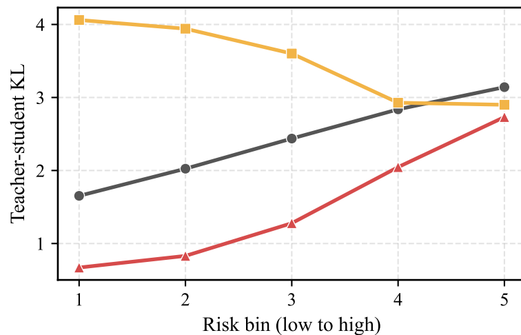
CINIC DenseNet121
