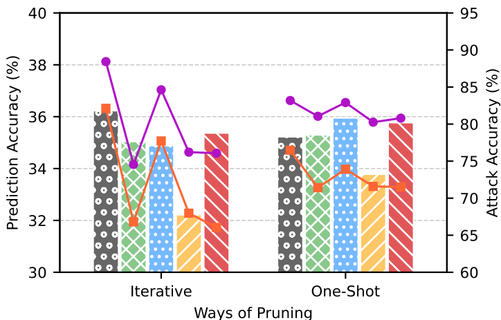
(a) CIFAR100 VGG16
