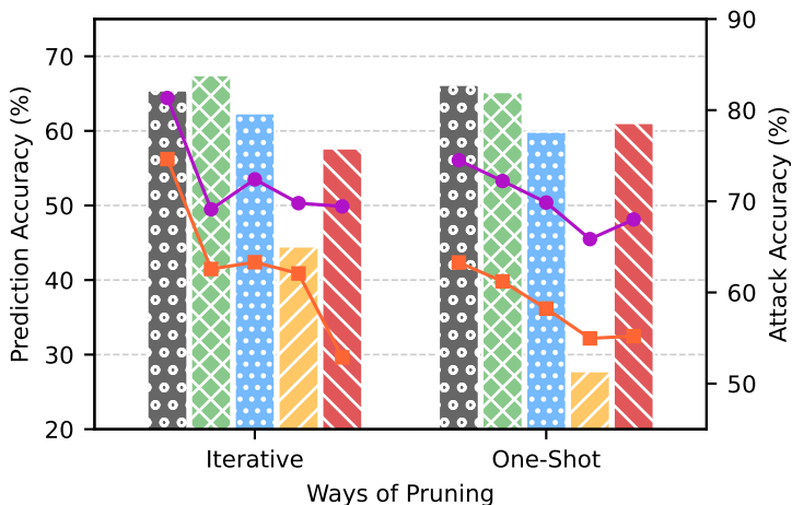
(c) RESISC45 ResNet18
