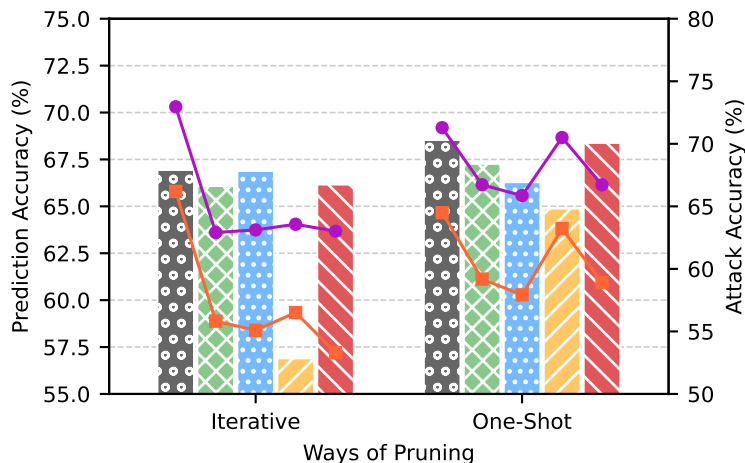
(b) CINIC DenseNet121
