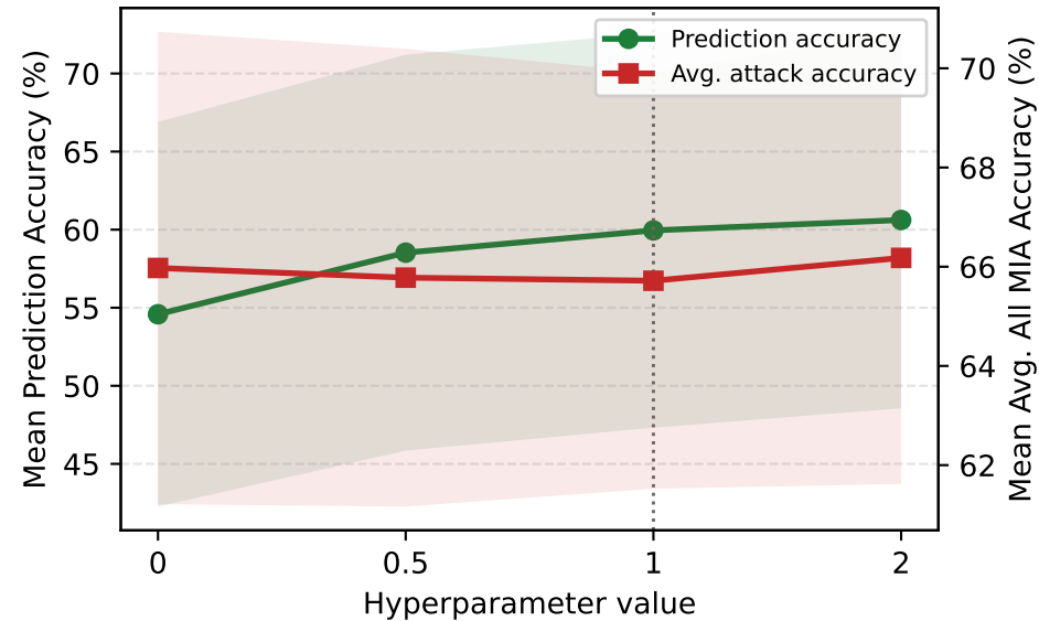
Distillation Weight
