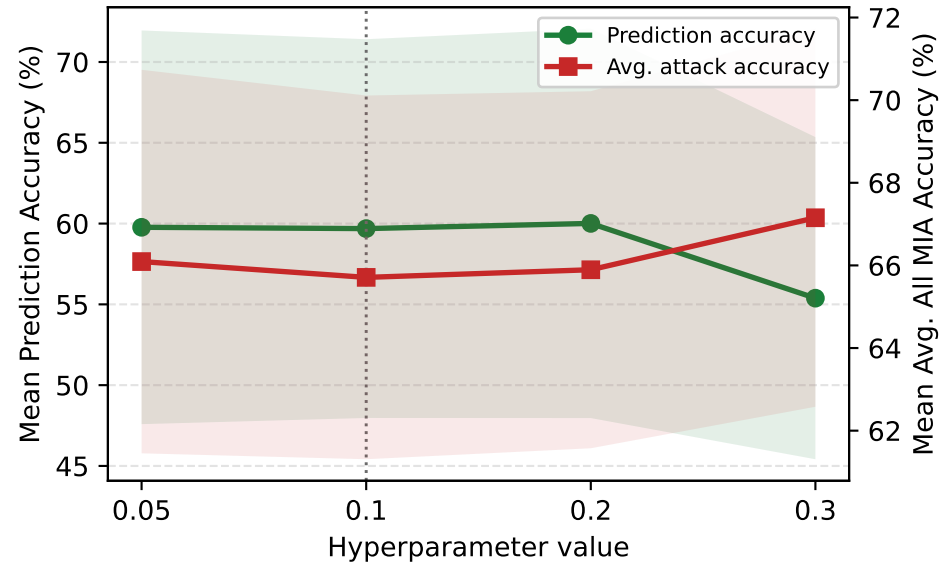
High-Risk Ratio
