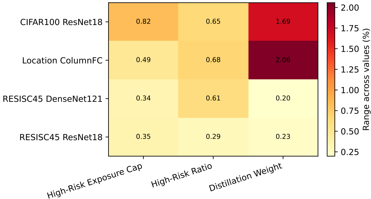
Attack Sensitivity Heatmap (Avg. All MIA Accuracy (%))
