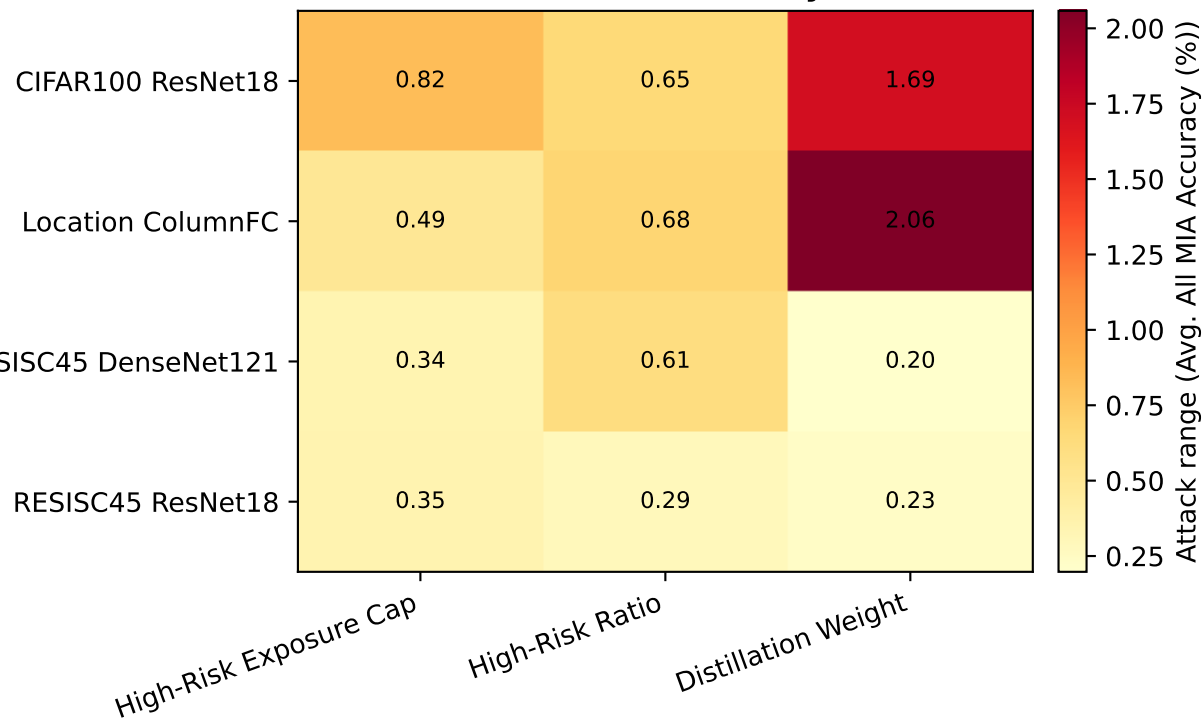
Attack Sensitivity
