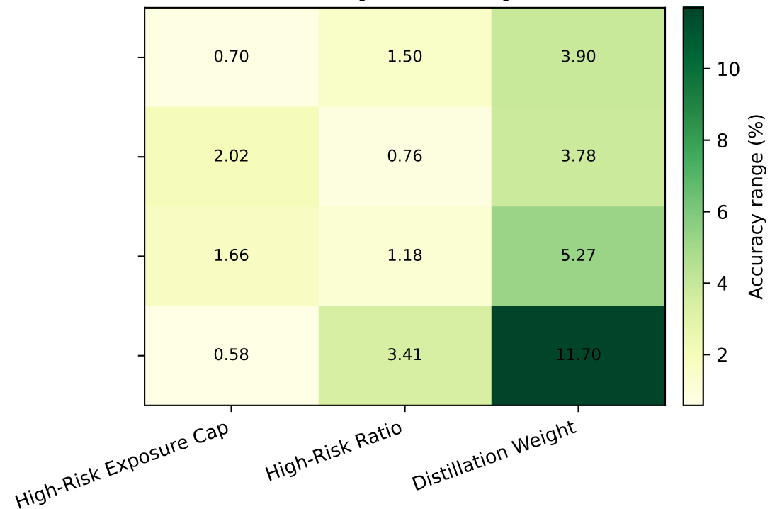
Utility Sensitivity
