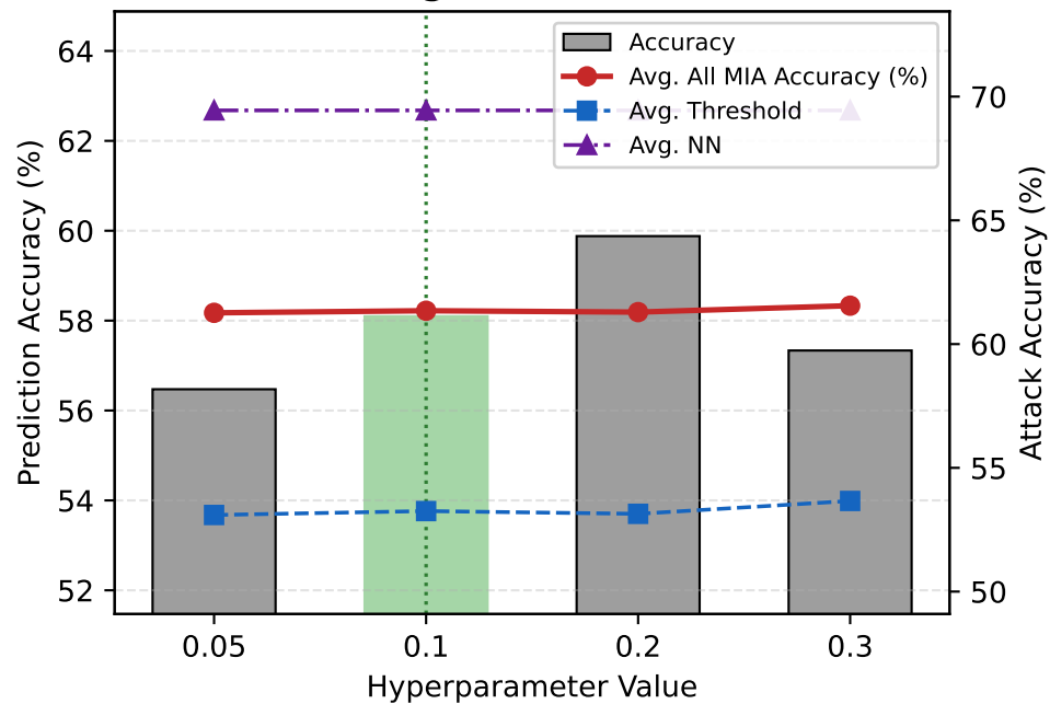
High-Risk Ratio
