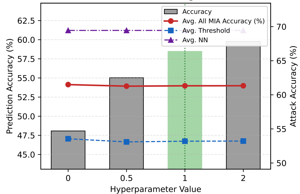
Distillation Weight
