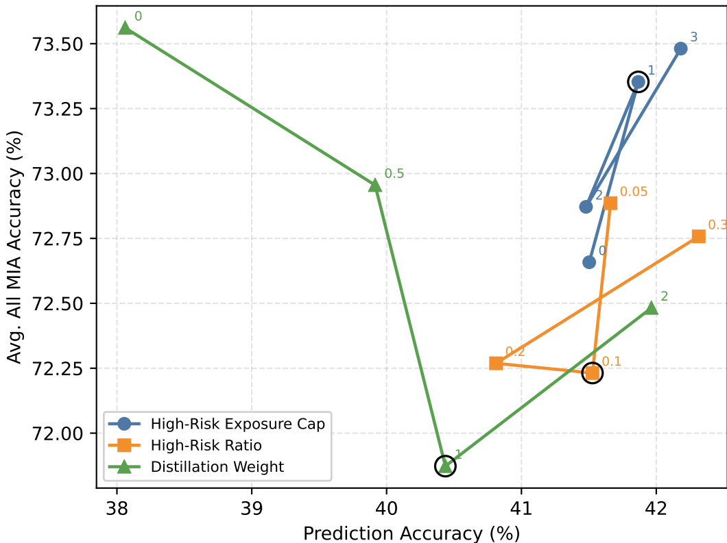
Privacy-Utility Trade-off: CIFAR100 ResNet18
