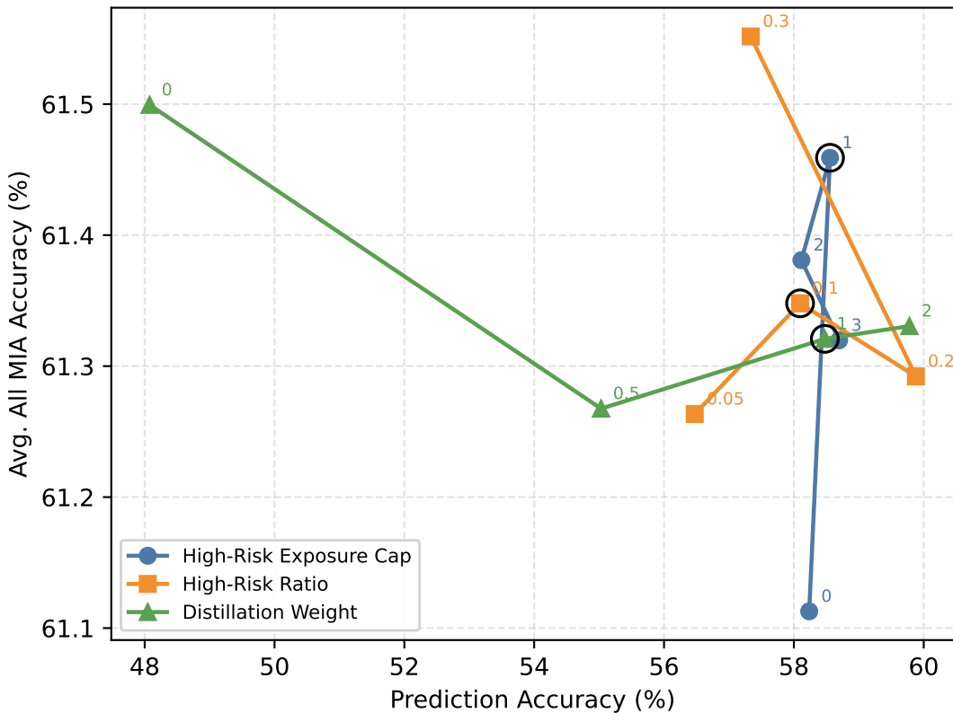
Privacy-Utility Trade-off: RESISC45 ResNet18
