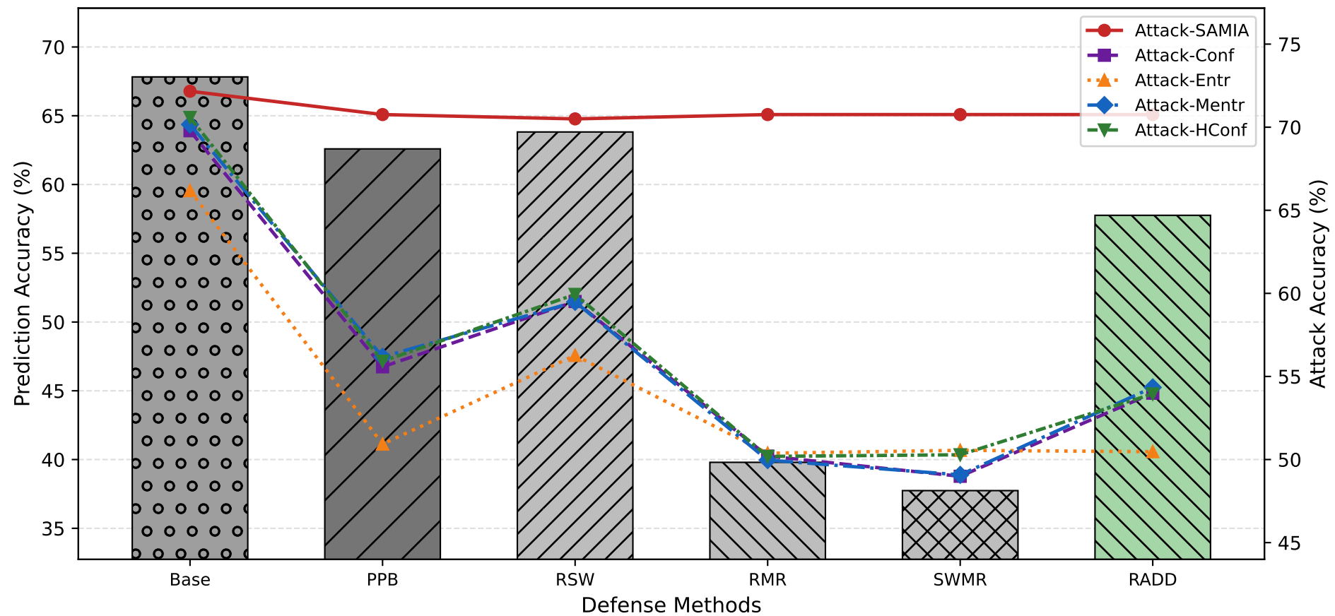
(Stl10 Resnet18)
