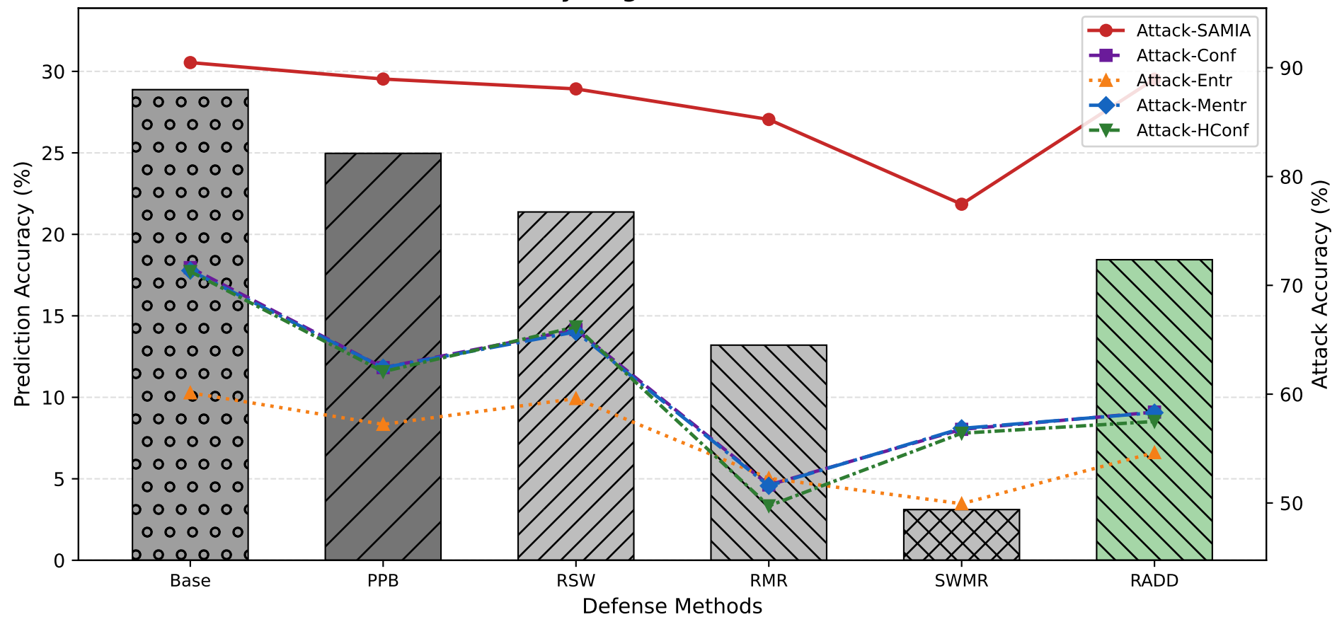
(Tinyimagenet Resnet18)
