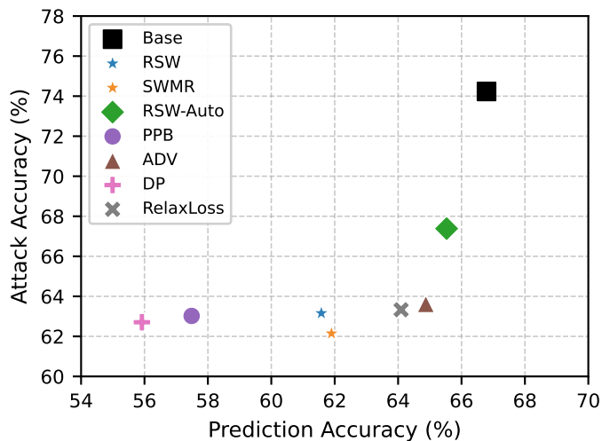
(c) VGG16 (SAMIA)
