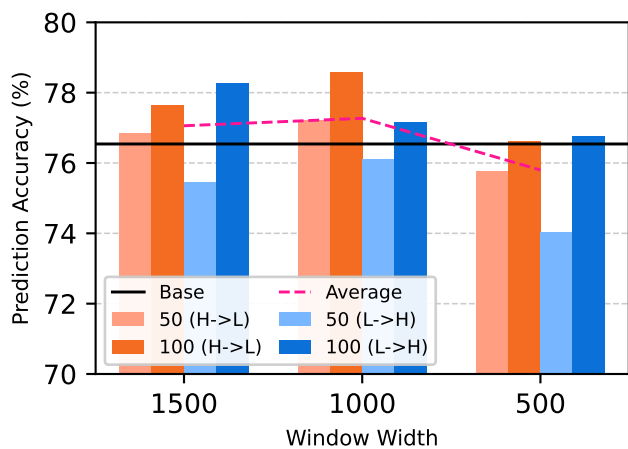
(a) CIFAR10 Res18 (RSW)
