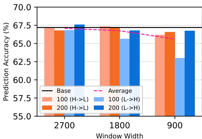
(e) CINIC VGG16 (RSW)
