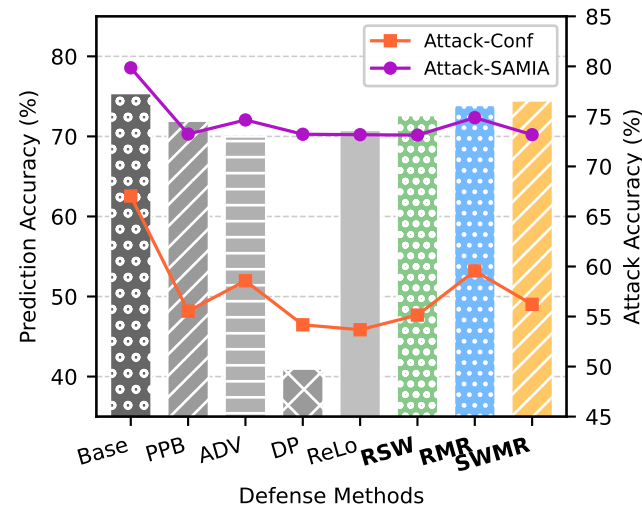
(a) CIFAR10 ResNet18
