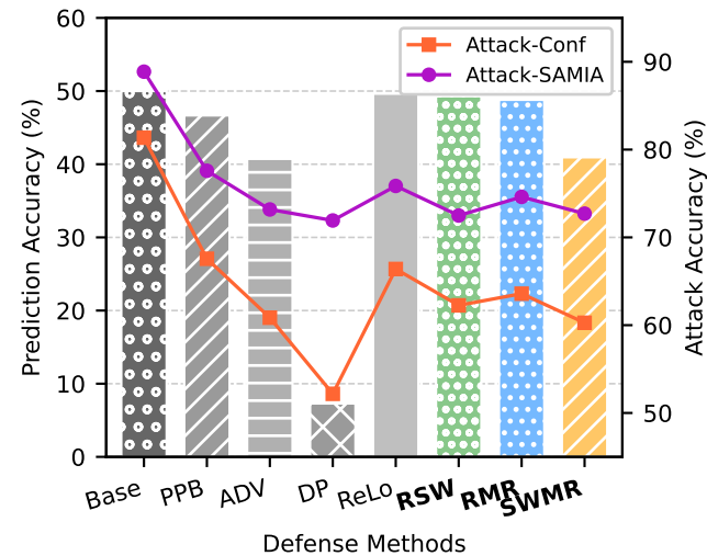
(b) CIFAR100 DenseNet121
