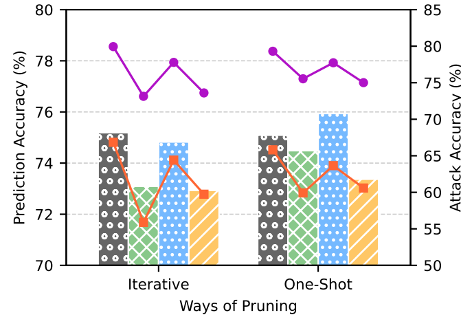
(a) CIFAR10 ResNet18
