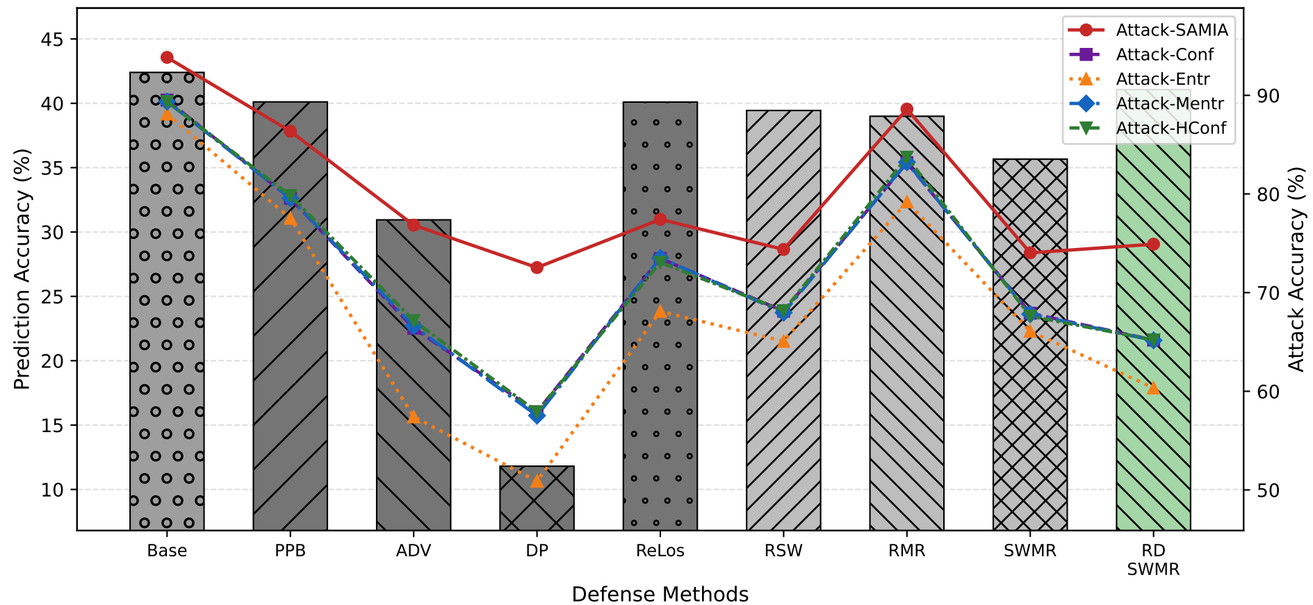
(Cifar100 Resnet18)
