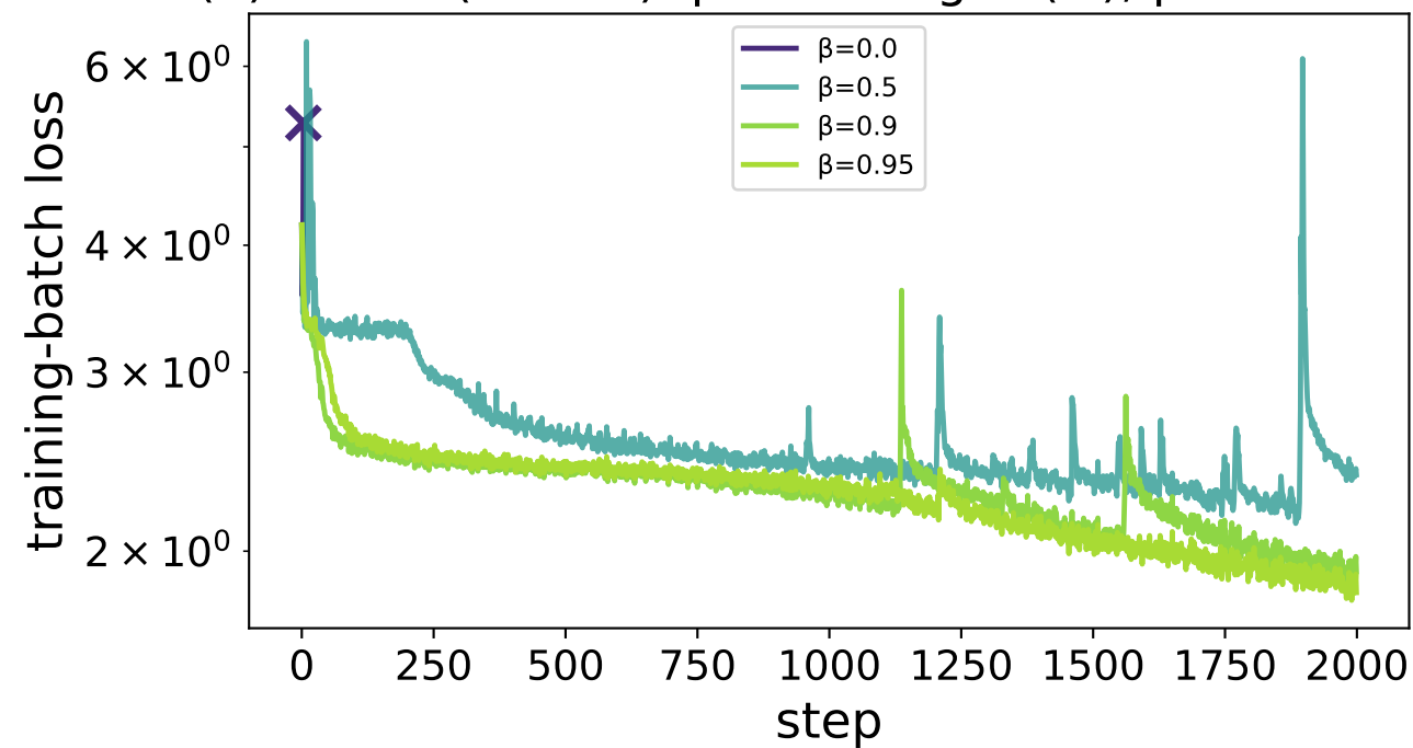
(b) Lr=0.4 (seed 0): \beta=0 diverges ( \times ), \beta \geq 0.9 trains
