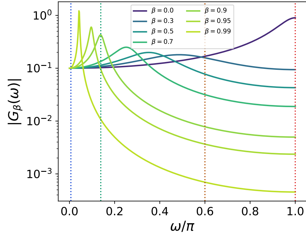
(c) closed-loop gain, arms dotted
