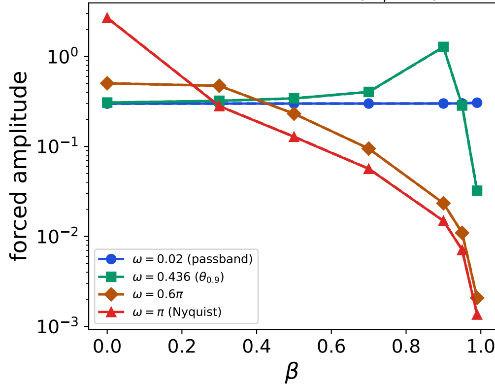
(b) amplitude on A |G_\beta(\omega)|
