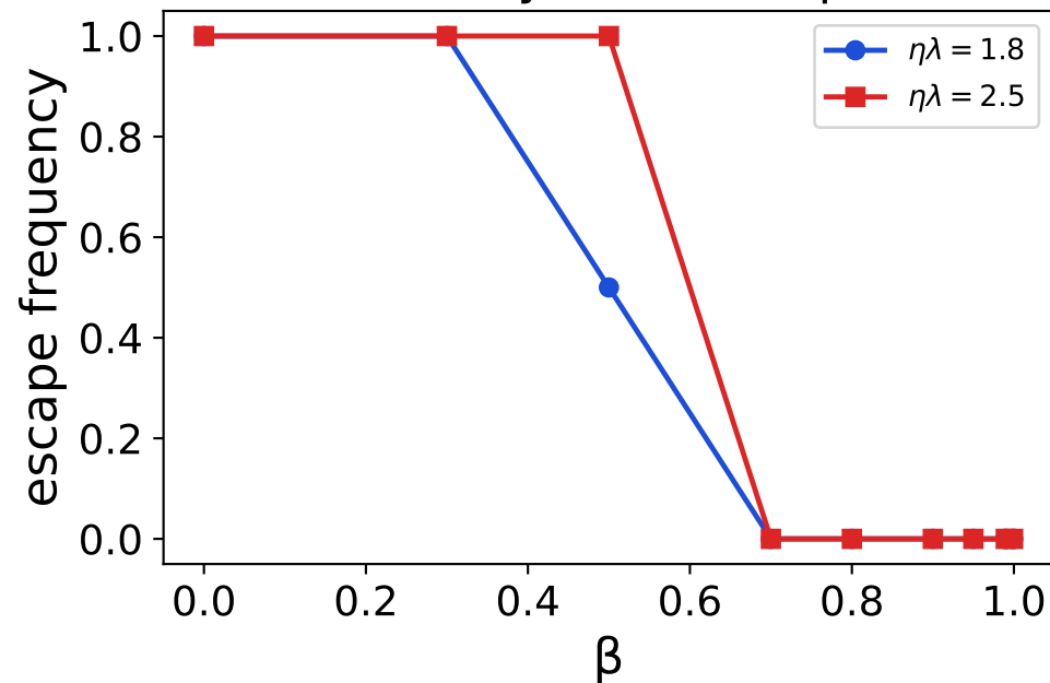
(b) curved valley: tube escape (R=2.0)
