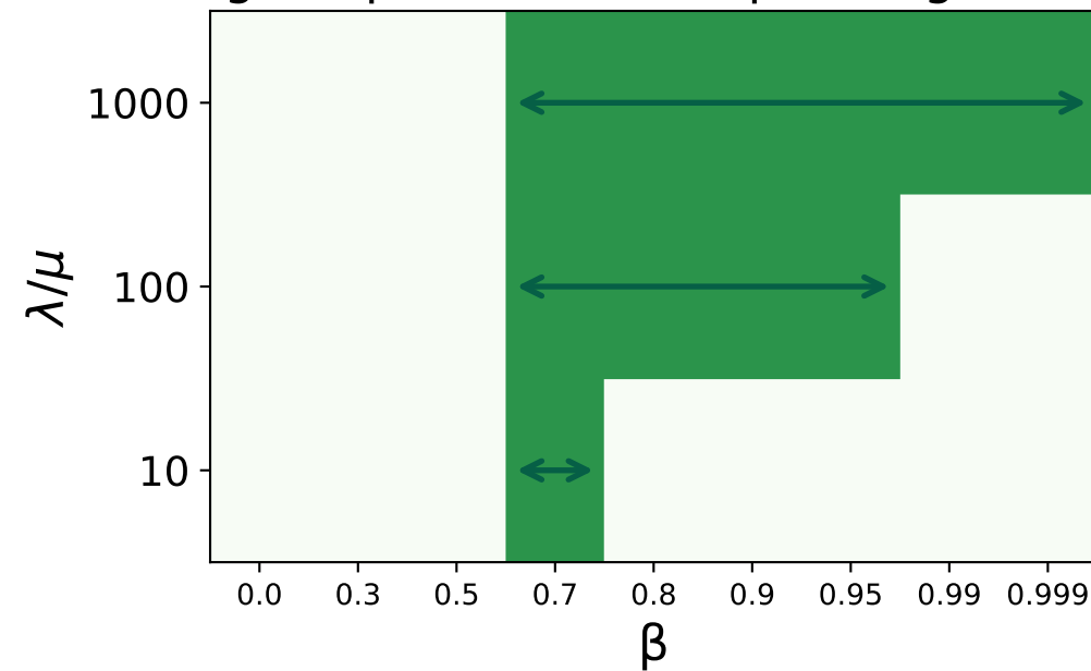
(c) good- \beta window (escape & lag criteria)
