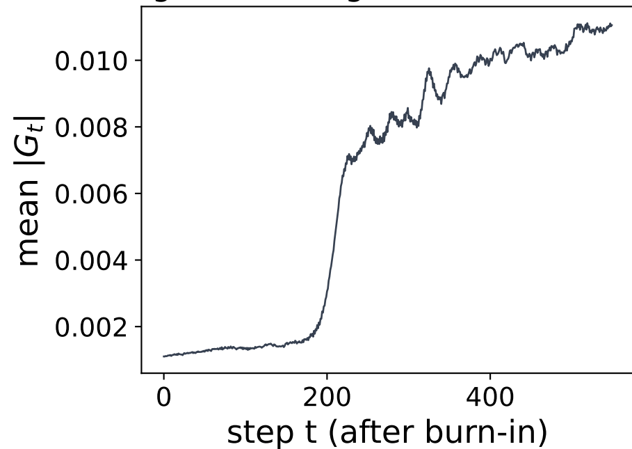
(a) gradient magnitude over training
