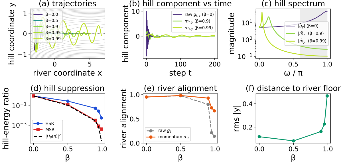
Figure 4: Straight river valley (E1), \beta \in \{0, 0.5, 0.9, 0.95, 0.99\} , \eta\lambda = 1.8 , T = 200 . (a) iterate trajectories on the loss contour. (b) hill component over time: raw g_{t,y} at \beta = 0 and momentum m_{t,y} at \beta \in \{0.9, 0.99\} . (c) temporal spectrum of the hill component (rectangular window), high band \omega \geq 0.6\pi shaded. (d) hill suppression ratio HSR and momentum suppression ratio MSR versus \beta with the |H_\beta(\pi)|^2 guide. (e) per-step river alignment of g_t and m_t , averaged over t . (f) rms distance to the river floor. Source: run straight_valley_trajectory_eta0p18_lam10_T200 .
