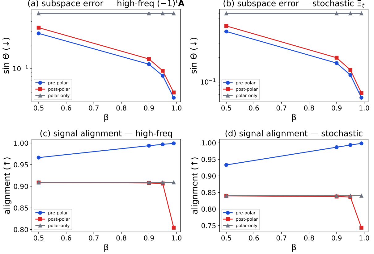
Figure 9: Filter-first on the matrix/Muon toy (E5), d_1=24, d_2=18, r=3, T = 400 . Subspace error \|\sin \Theta\|_2 (log, lower better) versus \beta for (a) the high-frequency disturbance and (b) the stochastic disturbance; rank- r signal alignment (higher better) versus \beta for (c) high-frequency and (d) stochastic. Series: pre-polar, post-polar, polar-only. Source: run matrix_muon_pipeline_m24n18r3_T400 .
