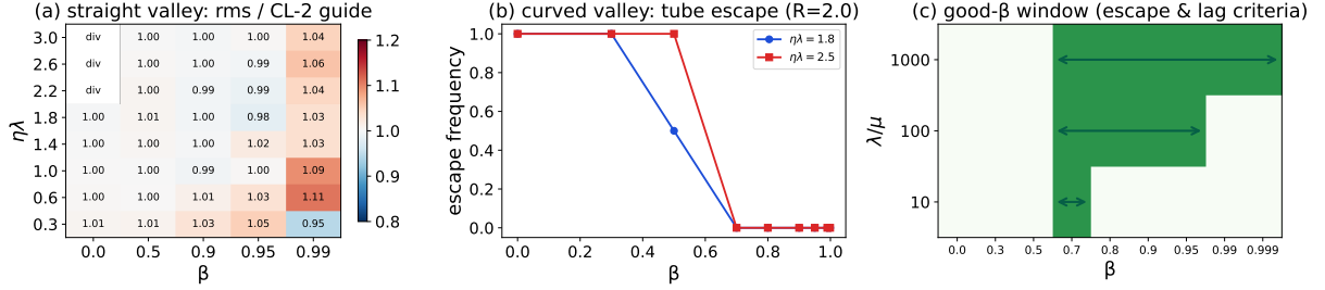
Figure 11: Closed-loop grid. (a) straight valley, \sigma = 2 , 8 seeds, T = 6000 : measured stationary rms over the Proposition 3 guide, per (\eta\lambda, \beta) cell; cells beyond the Proposition 2 threshold marked “div”. (b) curved valley, T = 300 : tube-escape frequency versus \beta at \eta\lambda \in \{1.8, 2.5\} , R = 2 . (c) \beta window (shaded, arrow-spanned) versus conditioning \lambda/\mu at \eta\lambda = 1.8 : escape frequency \leq 0.25 and mean river-following lag \leq 1.25 \times its per-conditioning minimum over the traveling horizon 3/(\eta\mu) , 16 seeds. Source: run c12_grid_sweep_e18_b5_seeds8.
