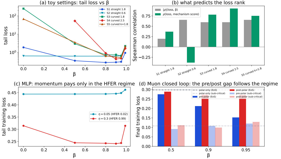
Figure 14: Optimizer-level tests (E7). (a) closed-loop EMA momentum tail loss versus \beta (log) on the five toy settings, \sigma = 2, 8 seeds; diverged cells omitted. (b) per-setting Spearman correlation of the tail-loss rank with \beta (grey, absolute value) and with the mechanism score (green). (c) the network of Section 9 trained closed-loop: tail training loss versus \beta at \eta \in \{0.05, 0.3\} , each regime’s stream HFER in the legend. (d) Muon-style pre-polar versus post-polar on the first layer at \eta = 0.3, \eta_o = 0.02 : final training loss by \beta . Sources: runs optimizer_toy_closedloop_set5_b6_seeds8 , optimizer_mlp_closedloop_eta2_b6_muon3 .
