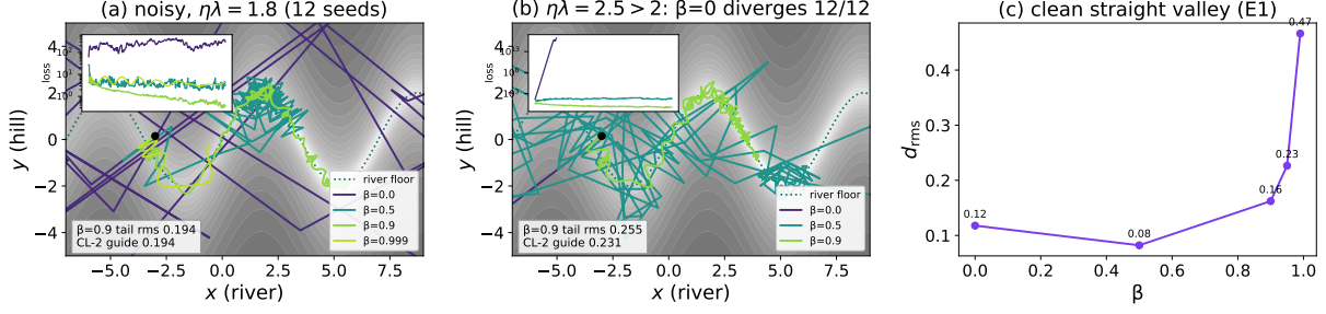
Figure 10: Regimes of momentum in the river valley (E8). Curved valley f(x) = 2 \sin(0.9x) , Gaussian gradient noise \sigma = 2 , T = 300 , 12 seeds; trajectories are seed 0 on the loss contour with the river floor dotted, insets are seed-mean loss (log). (a) \eta\lambda = 1.8 , \beta \in \{0, 0.5, 0.9, 0.999\} ; the annotation gives the \beta = 0.9 seed-mean tail rms of the hill offset against the Proposition 3 guide. (b) \eta\lambda = 2.5 , \beta \in \{0, 0.5, 0.9\} ; \beta = 0 diverges on all seeds ( \times marks the last finite point). (c) E1’s clean straight valley: d_{rms} versus \beta . Sources: runs valley_regimes_trajectory_eta0p18_0p25_sig2_seeds12_T300, straight_valley_trajectory_eta0p18_lam10_T200.
