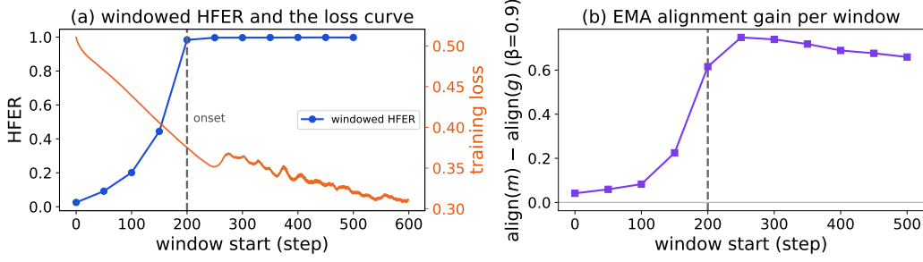
Figure 12: Confinement onset (E6), windows of length 100, stride 50, over the full 600-step stream. (a) windowed HFER per window start, training loss on the right axis, onset (first window with HFER \geq 0.9 ) dashed. (b) per-window alignment gain \text{Align}_{\text{slow}}(m) - \text{Align}_{\text{slow}}(g) at \beta = 0.9 against the window-mean gradient, first 20 in-window steps dropped as warm-up. Source: run mlp_diagnostic_trajectory_cond120_eta0p3_T600 .
