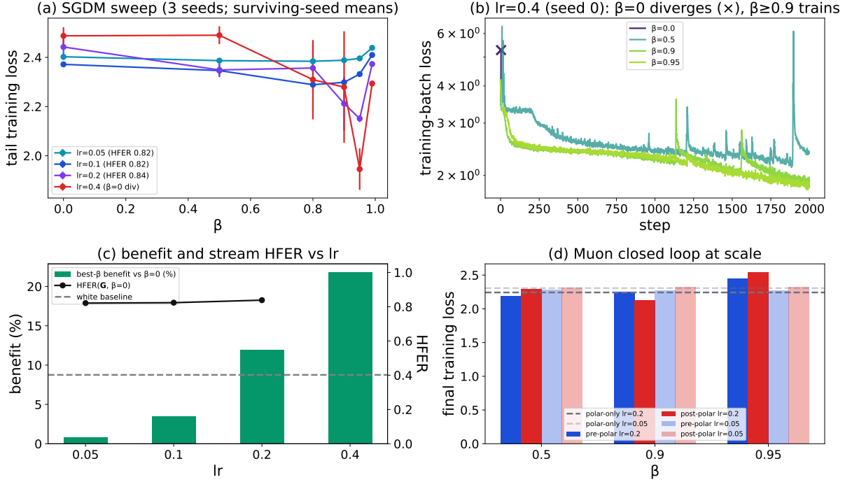
Figure 15: Mini-batch nanoGPT (E11): 0.40M-parameter character-level GPT (upstream nanoGPT, unmodified), shake-speare_char, batch 32 \times 128 , T = 2000 , EMA-SGDM on all parameters, no gradient clipping, 3 seeds with seed-fixed batch order; probe window steps 1200–1455 of the last block’s MLP expansion gradient. (a) tail training loss (mean of the last 200 steps) versus \beta per learning rate; surviving-seed means, error bars seed std; legend entries carry the raw-stream HFER at \beta = 0 . (b) seed-0 loss curves at lr = 0.4 ; \times marks the \beta = 0 divergence. (c) best- \beta benefit over \beta = 0 (bars) and HFER( \mathbf{G}, \beta=0 ) (line) versus learning rate, white-stream baseline dashed. (d) Muon pre-/post-polar final loss at background lr \in \{0.2, 0.05\} , \eta_o = 0.02 , polar-only dashed per lr . Source: run nanogpt_closedloop_lr4_b6_seeds3_T2000.
