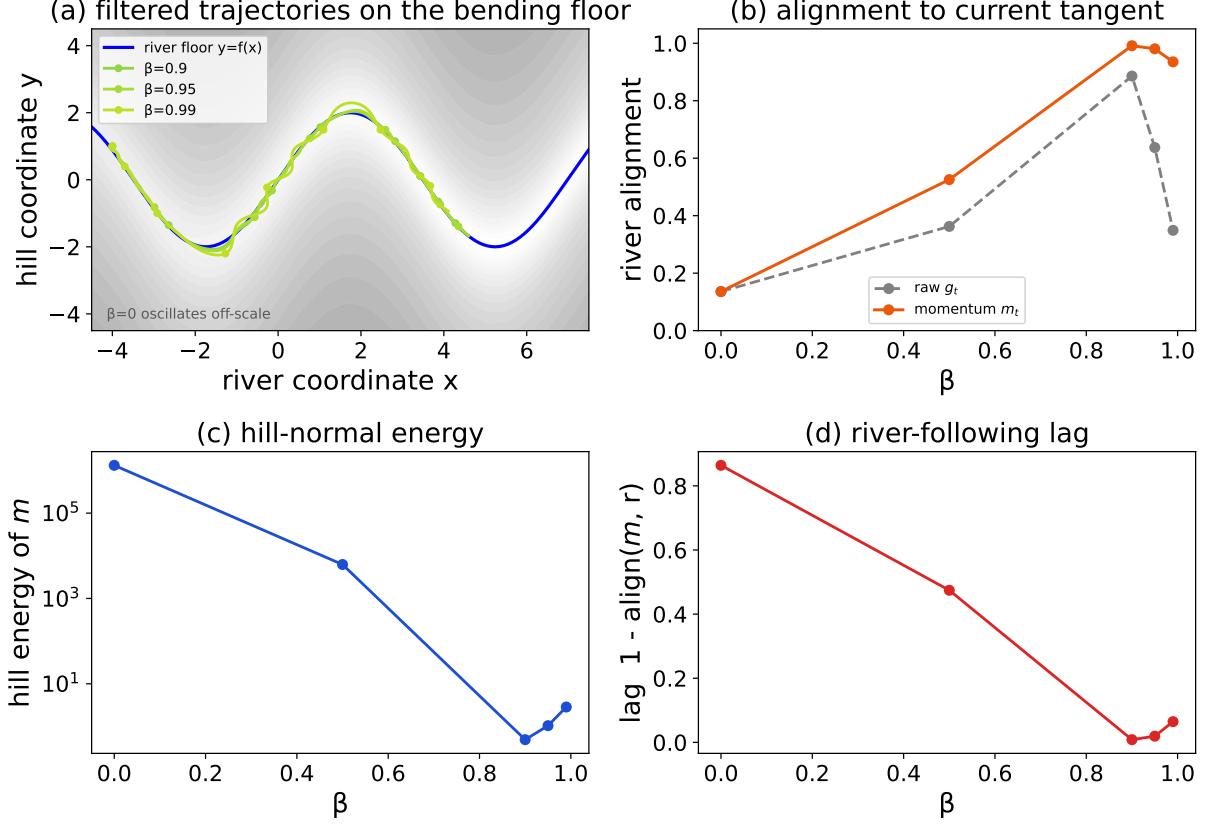
Figure 5: Curved river valley (E2), f(x) = 2 \sin(0.9x) , \eta\lambda = 1.8 , T = 300 . (a) filtered trajectories ( \beta \in \{0.9, 0.95, 0.99\} ) on the bending floor; the near-unstable \beta = 0 baseline is off-scale and quantified in (b)–(d). (b) river alignment of g_t and m_t versus \beta . (c) hill-normal energy of m_t versus \beta (log). (d) river-following lag 1 - \text{Align}_{\mathcal{R}}(m_t) versus \beta . Source: run curved_valley_trajectory_a2_k0p9_eta0p18_T300.
