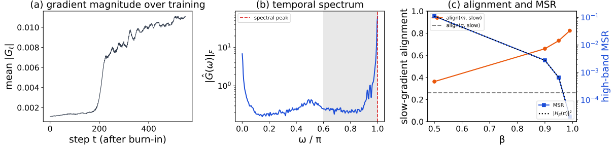
Figure 13: Real two-layer network at the edge of stability (E6), \eta = 0.3 , full-batch GD, T = 600 . (a) mean magnitude of the first-layer gradient over training. (b) temporal Frobenius spectrum, high band \omega \geq 0.6\pi shaded, dominant peak marked. (c) slow-gradient alignment of the EMA buffer versus \beta (left, with the raw-gradient baseline dashed) and high-band MSR with the |H_\beta(\pi)|^2 guide (right, log). Source: run_mlp_diagnostic_trajectory_cond120_eta0p3_T600 .
