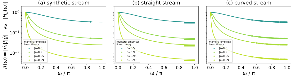
Figure 7: Empirical EMA transfer ratio versus theory (E4), T = 512 , Hann window. Each panel is a fixed input stream (synthetic, straight-valley hill, curved-valley hill); markers are the measured ratio |\hat{m}|/|\hat{g}| on significant-energy bins, solid lines are |H_{\beta}(\omega)| , for \beta \in \{0.5, 0.9, 0.95, 0.99\} (log). Source: run frequency_validation_spectral_T512_hann .
