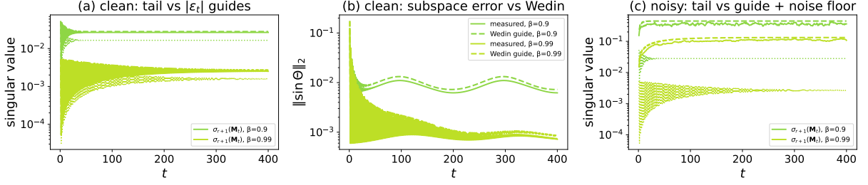
Figure 8: Constants of Theorem 4 on the matrix/Muon toy (E5 overlay), d_1=24, d_2=18, r=3, T=400, \beta \in \{0.9, 0.99\} . (a) noise-free scenario: measured \sigma_{r+1}(\mathbf{M}_t) (solid) against the upper guide |\varepsilon_t|\|\mathbf{A}\|_2 (dashed) and lower guide |\varepsilon_t|\sigma_{2r+1}(\mathbf{A}) (dotted), log scale. (b) noise-free scenario: measured subspace error (solid) against the bound of Theorem 4(b) (dashed). (c) noisy scenario ( \sigma_\xi = 0.2 ): measured tail against the deterministic guide (dotted) and the guide plus the iid-Gaussian operator-norm floor (dashed). Source: run matrix_muon_pipeline_m24n18r3_T400 .
