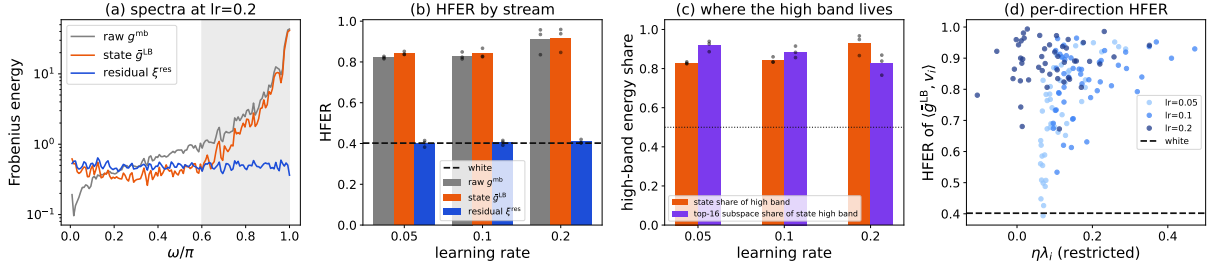
Figure 16: Decomposition of the mini-batch stream (E12), nanoGPT probe window as in Figure 15, plain SGD, 3 seeds, large-batch size 1024, k = 16 eigenpairs. (a) per-frequency Frobenius energy of g^{\text{mb}} , g^{\text{LB}} , \xi^{\text{res}} at \text{lr} = 0.2 , seed mean (log). (b) HFER of the three streams per learning rate, white baseline dashed. (c) high-band state share and, of the state stream, the share captured by the top-16 curvature subspace, per learning rate. (d) per-direction HFER of the state stream’s coefficient series against \eta\lambda_i (restricted eigenvalues), all learning rates and seeds, white baseline dashed. Source: run nanogpt_decomp_lr3_seeds3_LB1024_k16.
