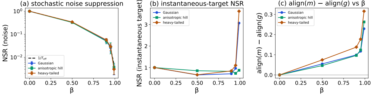
Figure 6: Noisy straight valley (E3), 12 seeds, \sigma = 2 . (a) noise suppression ratio NSR versus \beta for three noise models with the 1/T_{\text{eff}} floor (log, error bars are seed std). (b) instantaneous-target ratio versus \beta . (c) river-alignment difference \text{Align}_{\mathcal{R}}(m) - \text{Align}_{\mathcal{R}}(g) versus \beta . Source: run noisy_valley_trajectory_sig2p0_seeds12_eta0p18 .
