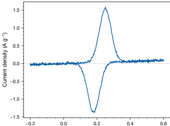
Fig 2. CV at 5 mV s -1 (Potential (V vs. ref.) - three cycles overlaid).
