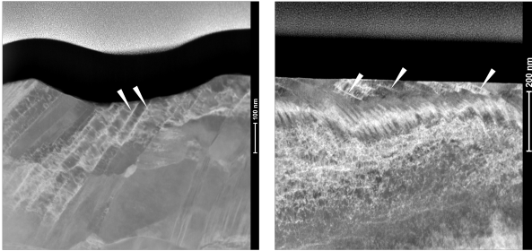
Cross-sectional STEM of conditioned hard (as-machined) Cu: dislocation-denuded zone in the top ~200 nm.
