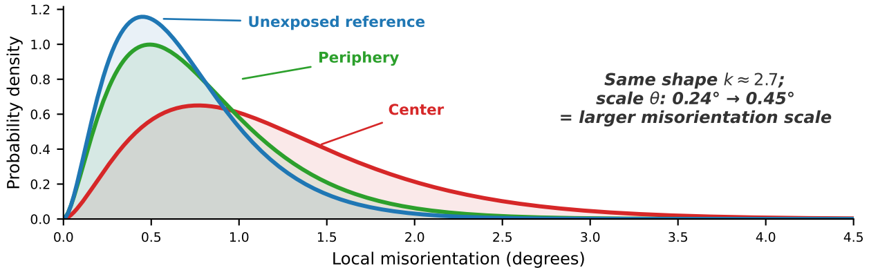
(c) Misorientation distributions broaden with field exposure
