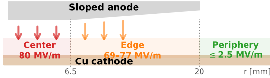
(a) Sloped-anode geometry
