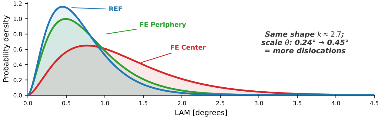
(c) Misorientation distributions broaden with field exposure
