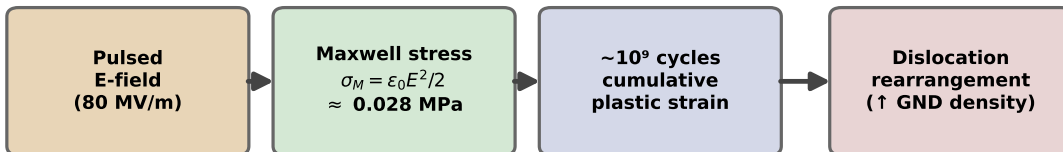
(d) Conditioning mechanism — from field to dislocation evolution
