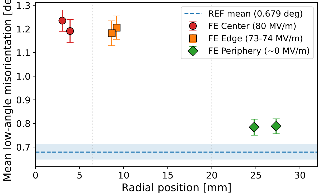
Mean intragrain misorientation vs. radial position on FE cathode
