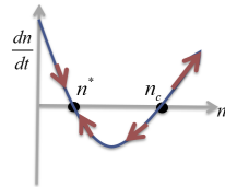
mobile-dislocation runaway
