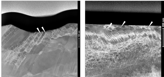
Cross-sectional STEM of conditioned hard (as-machined) Cu: dislocation-poor zone in the top ~200 nm.
