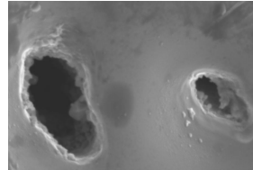
#3-25 field-exposed: “exploded” (HFW 10 \mu\text{m} )
