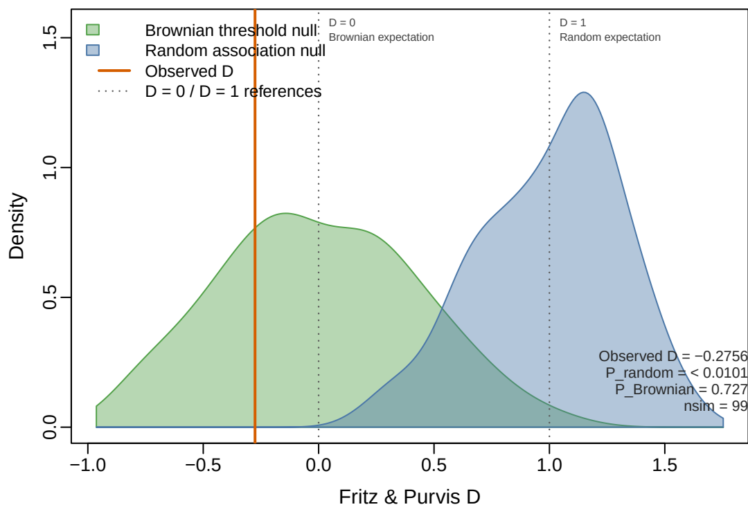
D calibration: Brownian and random nulls
