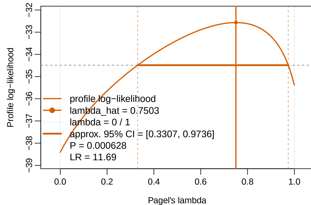
Pagel's lambda profile likelihood
