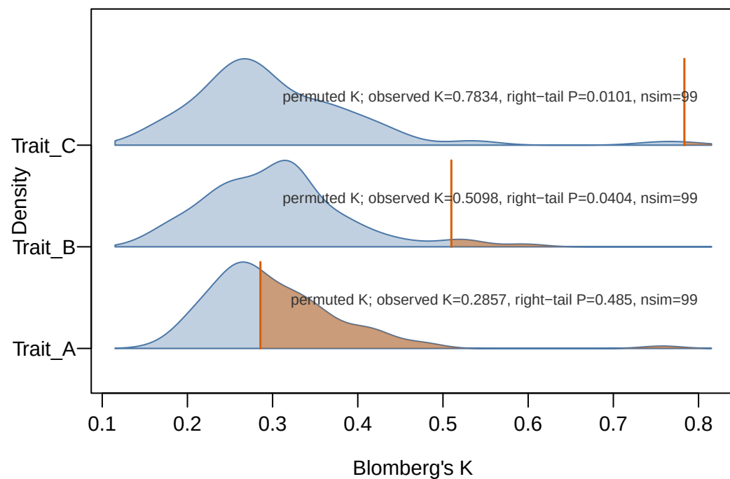
K permutation nulls: multiple traits
