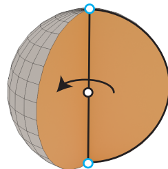
(c) Sphere
