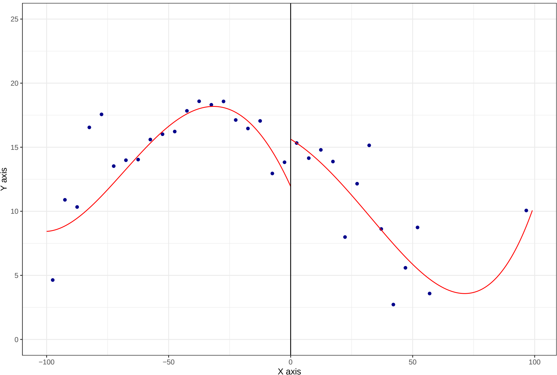
RD Plot
