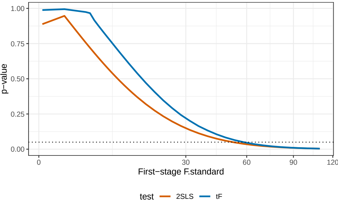
P-values vs First-Stage Strength
