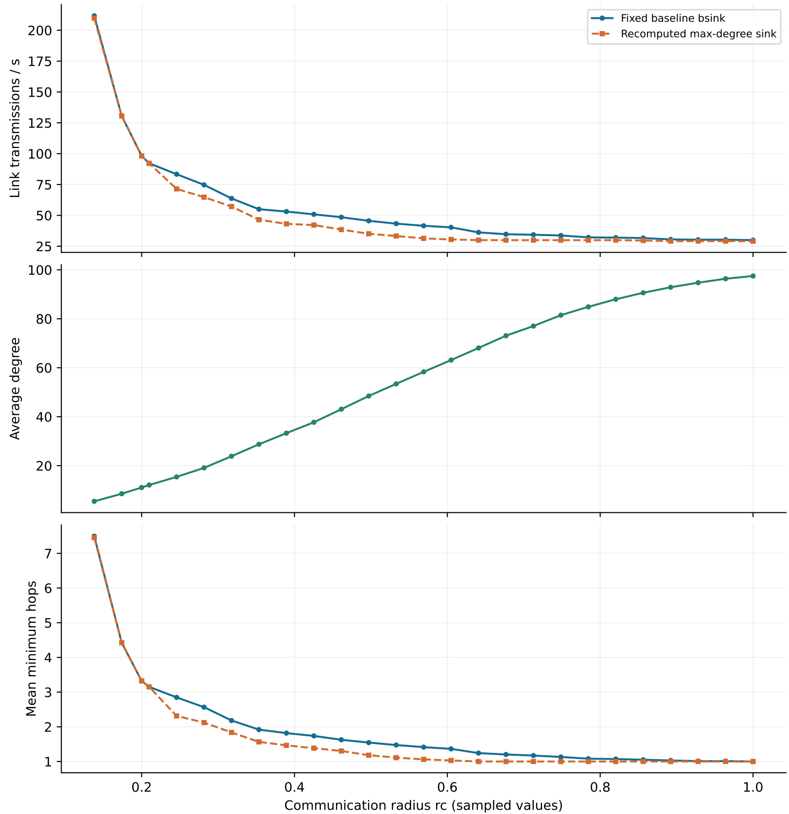
Q1b | Same positions and transmission periods
