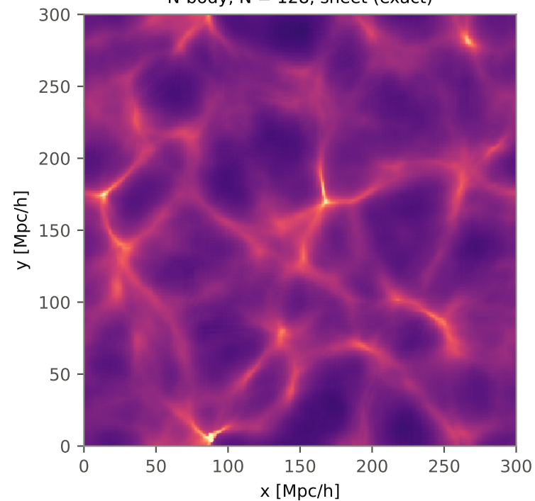
N-body, N = 128 , sheet (exact)
