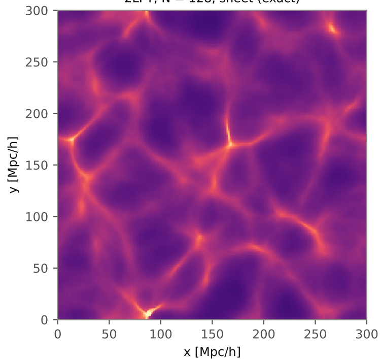
2LPT, N = 128 , sheet (exact)
