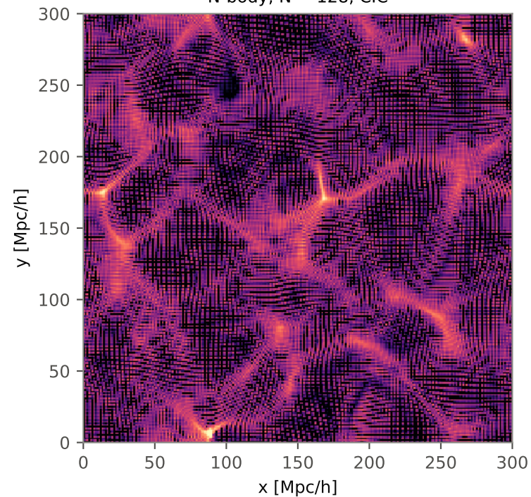
N-body, N = 128 , CIC
