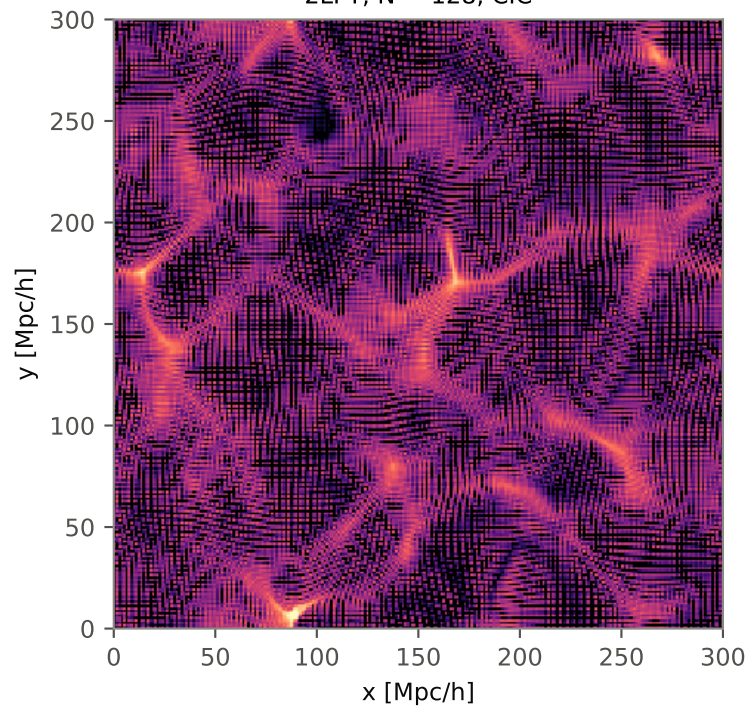
2LPT, N = 128 , CIC
