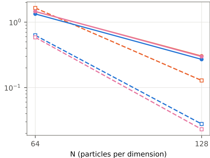
R_s = 14 Mpc/h, volume-weighted
