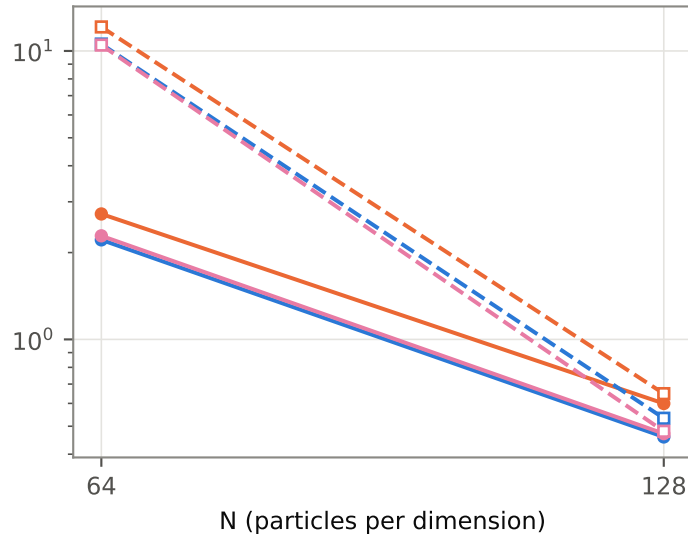
R_s = 7 Mpc/h, volume-weighted
