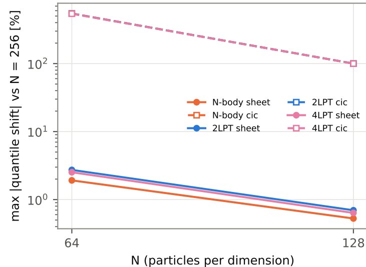
raw 1.17 Mpc/h cells, volume-weighted
