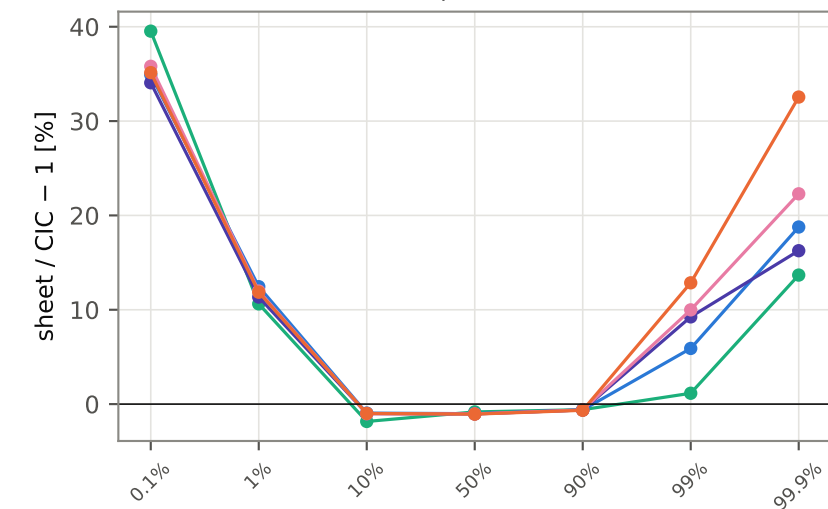
raw 1.17 Mpc/h cells (mass)
