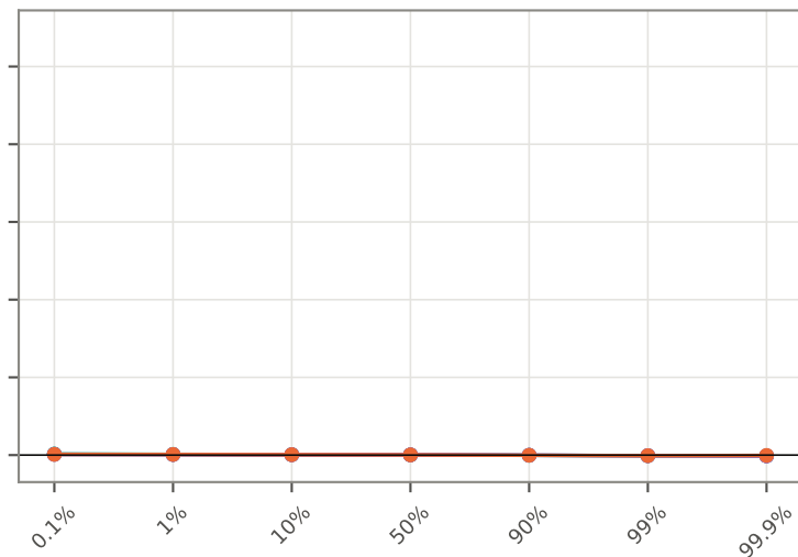
R_s = 7 Mpc/h (mass)
