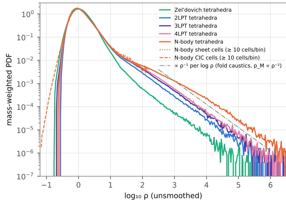
unsmoothed: tetrahedron stream density vs 1.17 Mpc/h cells
