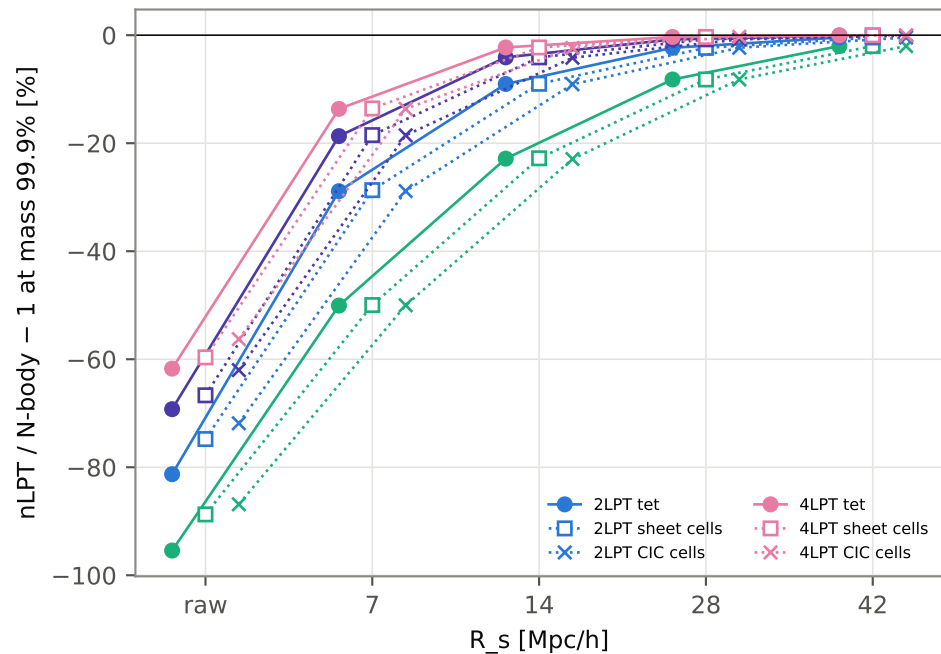
dense tail, three mass weightings
