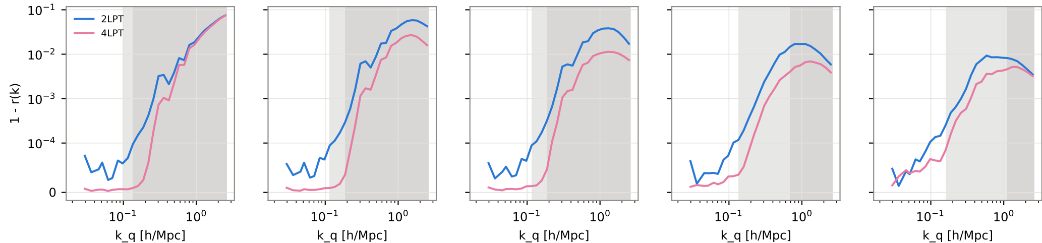
Step 2: cross-correlation of LPT and N-body scores, mass-weighted, z = 0 . Grey: unconverged. Conditional on the single-stream mask (both runs); not an unconditional two-point statistic.
