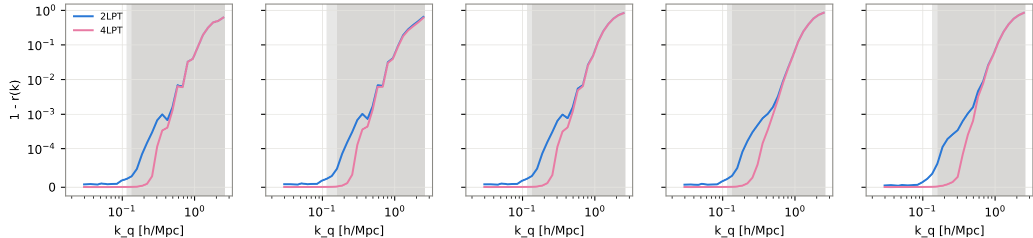
Step 2: cross-correlation of LPT and N-body scores, vol-weighted, z = 1 . Grey: unconverged. Conditional on the single-stream mask (both runs); not an unconditional two-point statistic.
