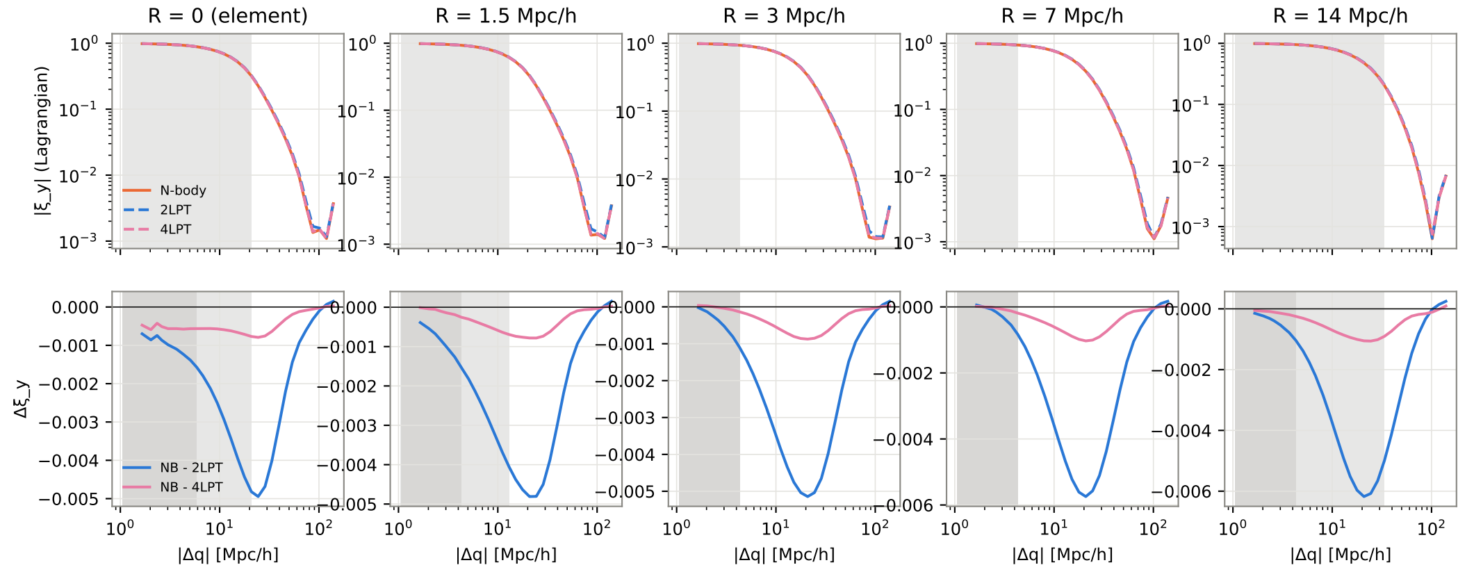
Step 2: Lagrangian copula \xi_y , mass-weighted, z = 0 , N = 256 . Grey: unconverged. Conditional on the single-stream mask (both runs); not an unconditional two-point statistic.
