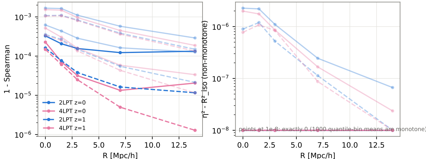
Step 3: element-paired ranks, mass-weighted (faint: lower N). Conditional on the single-stream mask (both runs); not an unconditional two-point statistic.
