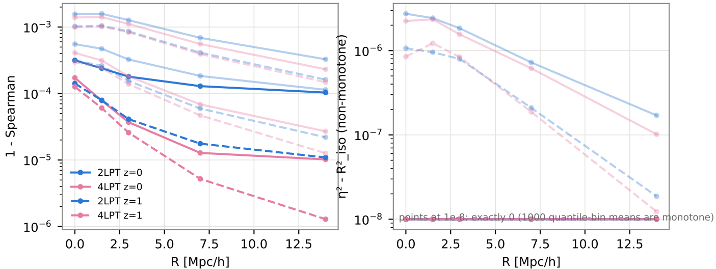
Step 3: element-paired ranks, vol-weighted (faint: lower N). Conditional on the single-stream mask (both runs); not an unconditional two-point statistic.
