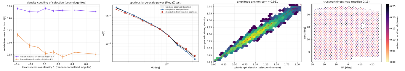
FIG. 12.— Completion diagnostics. Left : the spectroscopic success fraction as a function of the local target overdensity for the two missing-target kinds. Redshift failures are consistent with no density coupling ( h = -0.06 \pm 0.06 ), whereas fiber collisions are coupled ( h = -0.24 \pm 0.03 ) because close pairs occur in denser environments; since the completion places collided galaxies at their true imaging positions, this coupling is reproduced by construction rather than modeled. Right : the trustworthiness map — the galaxy-count scatter across completion realizations, per sky cell (median 0.13), which marks where the redshift posterior leaves the most freedom and the completion is extrapolating most strongly. CMASS-South is small enough to solve carefully and mature enough to validate against the standard answer; it is therefore a useful prototype for how future public survey products can serve both standard and beyond-two-point cosmology.
