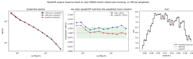
FIG. 10.— The default KNN-field redshift engine versus the graphGP conditional-field route, on the real CMASS-South data. Left: projected and angular clustering of the two completions against the official w_c -weighted reference; graphGP, being a smooth field draw, sits closer to the weighted reference on larger projected scales (ratio near unity), while the KNN-field realization is modestly high in some bins. Right: truth-known recovery of w_p(r_p) for both engines; the KNN-field engine is sharper on the sub-Mpc fiber-collision scale because it uses nearby observed redshifts directly, whereas graphGP is smoother and slightly closer on larger scales. Both recover the input clustering to the percent level; neither dominates, and the cheaper KNN-field route — which compresses to the public posterior — is the default.
