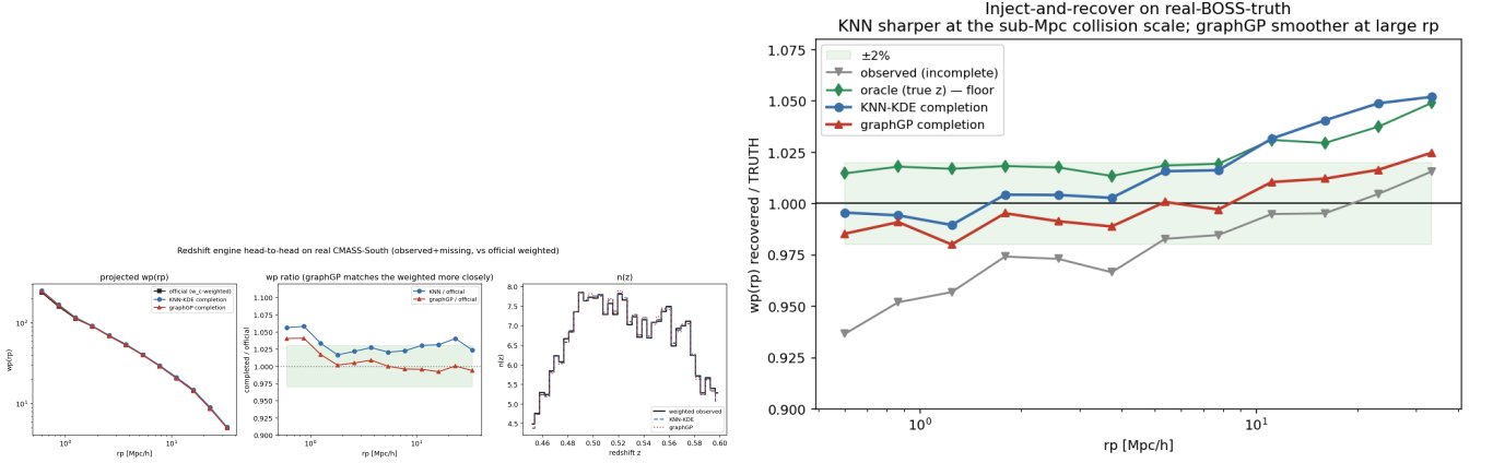
FIG. 11.— The default KNN-field redshift engine versus the graphGP conditional-field route, on the real CMASS-South data. Left : projected and angular clustering of the two completions against the official w_c -weighted reference; graphGP, being a smooth field draw, sits closer to the weighted reference on larger projected scales (ratio near unity), while the KNN-field realization is modestly high in some bins. Right : truth-known recovery of w_p(r_p) for both engines; the KNN-field engine is sharper on the sub-Mpc fiber-collision scale because it uses nearby observed redshifts directly, whereas graphGP is smoother and slightly closer on larger scales. Both recover the input clustering to the percent level; neither dominates, and the cheaper KNN-field route — which compresses to the public posterior — is the default.
