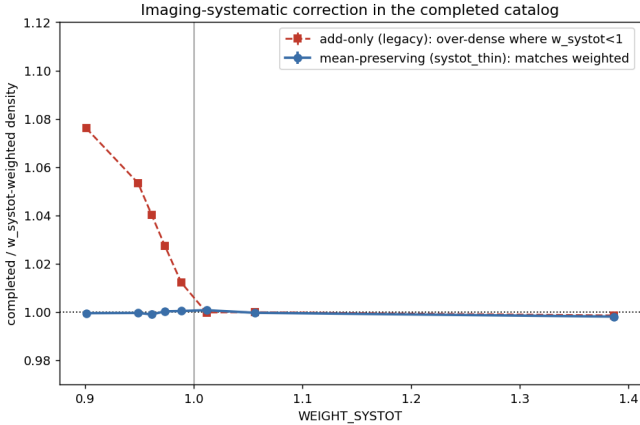
FIG. 3.— Mean-preserving imaging-systematic completion. The completed number density per w_{\text{SYSTOT}} bin, divided by the w_{\text{SYSTOT}} -weighted target density (isolating the systematic step on real CMASS-South). The mean-preserving completion (blue) reproduces the weighted density to \lesssim 0.2\% across the full range, whereas restoring the deficit without thinning the w_{\text{SYSTOT}} < 1 regions (red) leaves them over-dense by up to \sim 8\% , a residual degree-scale gradient correlated with the imaging systematic.
