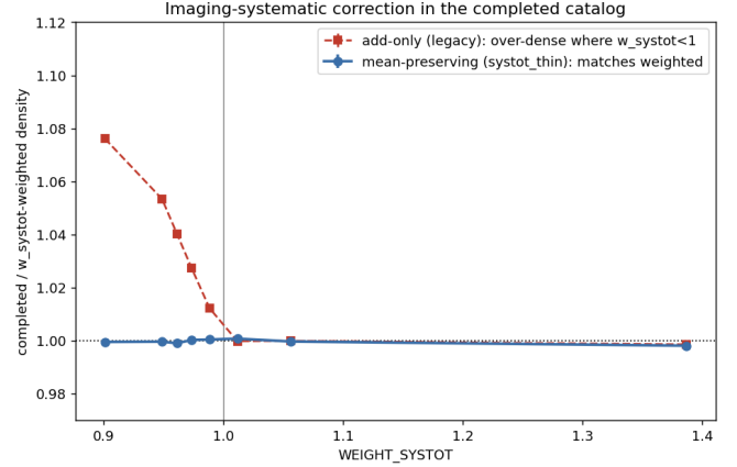
FIG. 3.— Mean-preserving imaging-systematic completion. The completed number density per w_{SYSTOT} bin, divided by the w_{SYSTOT} -weighted target density (isolating the systematic step on real CMASS-South). The mean-preserving completion (blue) reproduces the weighted density to \lesssim 0.2\% across the full range, whereas restoring the deficit without thinning the w_{SYSTOT} < 1 regions (red) leaves them over-dense by up to \sim 8\% , a residual degree-scale gradient correlated with the imaging systematic.
