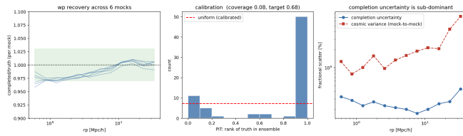
FIG. 9.— Calibration of the completion uncertainty against mock sample variance (MultiDark-Patchy). Per r_p bin, the realization-to-realization spread of the completed w_p(r_p) (the completion uncertainty) is 0.17–0.44%, well below the 0.8–7.2% sample variance, so the completion adds only 6–36% of the sample-variance error in quadrature. Because the ensemble conditions on the single observed CMASS-South realization and resamples only the unobserved spectroscopic information, it is deliberately narrow and must be added to a cosmic-variance or simulation covariance, not used in place of it.
