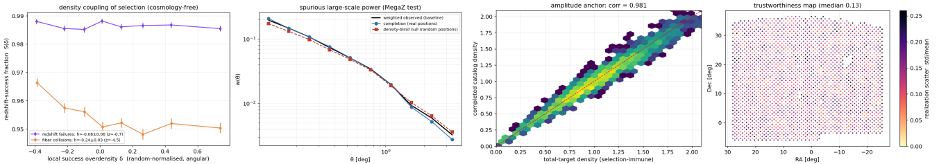
FIG. 11.— Completion diagnostics. Left : the spectroscopic success fraction as a function of the local target overdensity for the two missing-target kinds. Redshift failures are consistent with no density coupling ( h = -0.06 \pm 0.06 ), whereas fiber collisions are coupled ( h = -0.24 \pm 0.03 ) because close pairs occur in denser environments; since the completion places collided galaxies at their true imaging positions, this coupling is reproduced by construction rather than modeled. Right : the trustworthiness map — the galaxy-count scatter across completion realizations per sky cell (median 0.13) — which marks where the redshift posterior leaves the most freedom and the completion is extrapolating most strongly.
