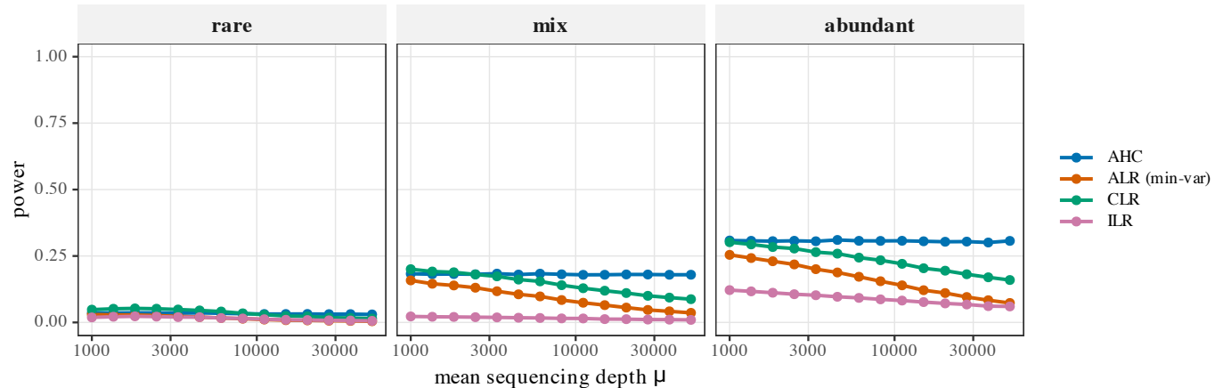
Differential abundance: power vs depth by signal location
